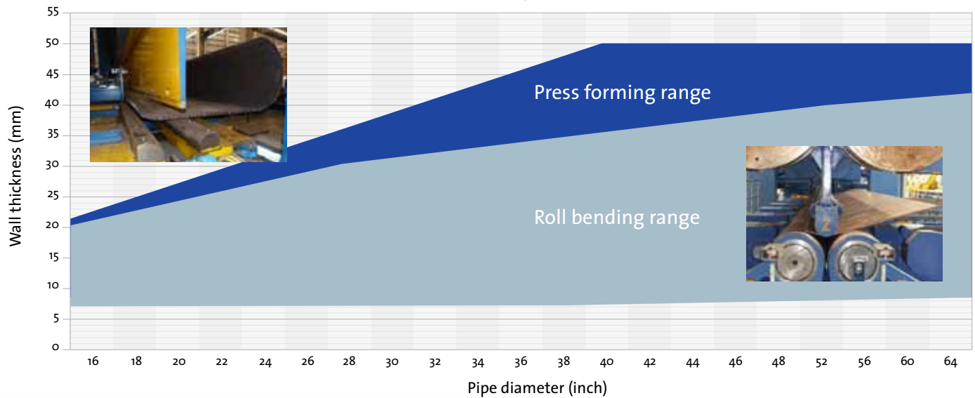
General capacity of HHT and overview of the two bending processes
